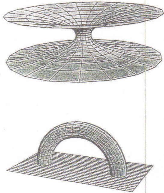
Figure 2. Inter-Universe Wormhole (top) and Intra-Universe Wormhole (bottom).
